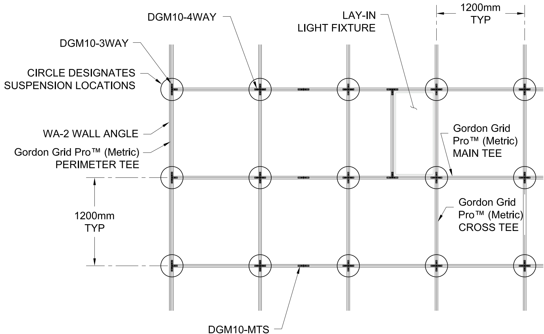
TYPICAL GRID PLAN NOT TO SCALE
